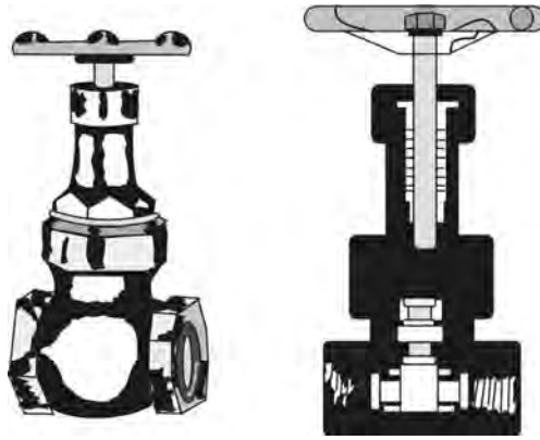
Figure 31 Gate valve
