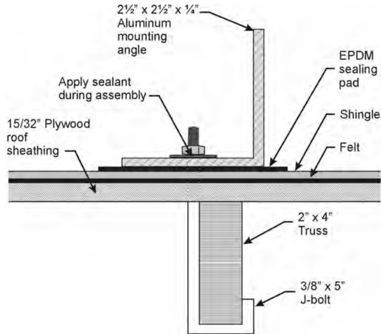
Figure 17 J-bolt mounting
