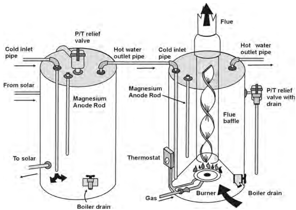
Figure 3 Gas heater connection
