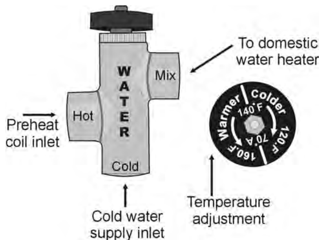
Figure 36 Tempering valve
