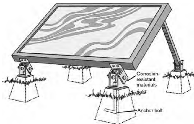
Figure 4 Ground mount
