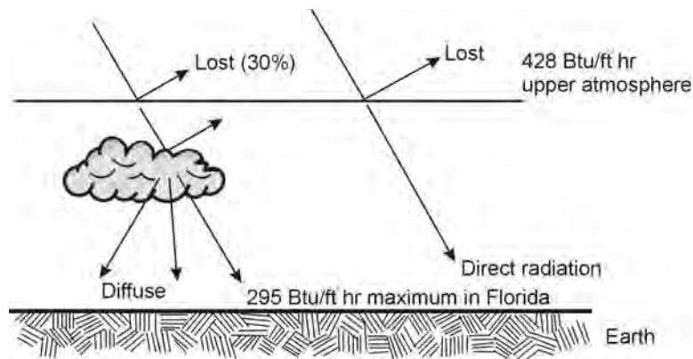
Figure 2. Atmospheric Effects on Solar Energy Reaching Earth
