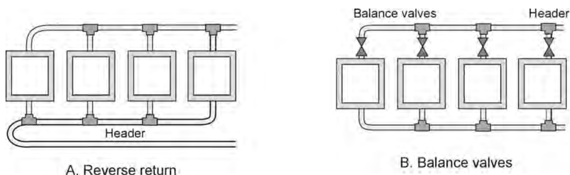
Figure 25 Multiple collector piping arrangements
