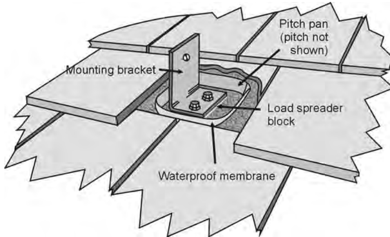
Figure 19 Mounting bracket for tile roofs
