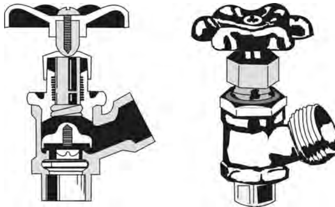
Figure 32 Drain valve
