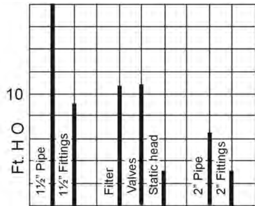
Figure 13 Relative pressure
