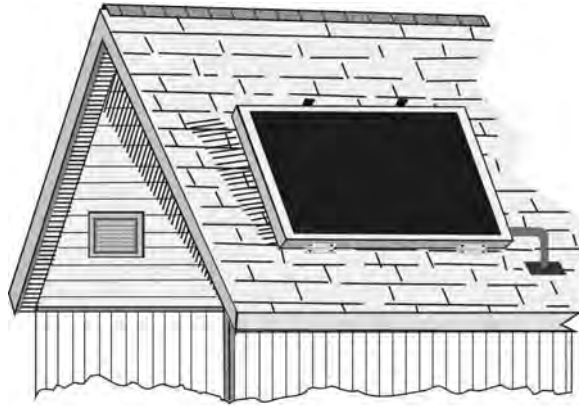
Figure 3 Collector mounted down from roof ridge to reduce wind loading and heat losses
