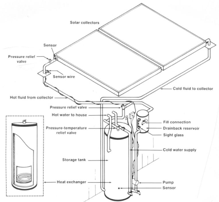
Figure 13 Drain-back system with internal tank heat exchanger
