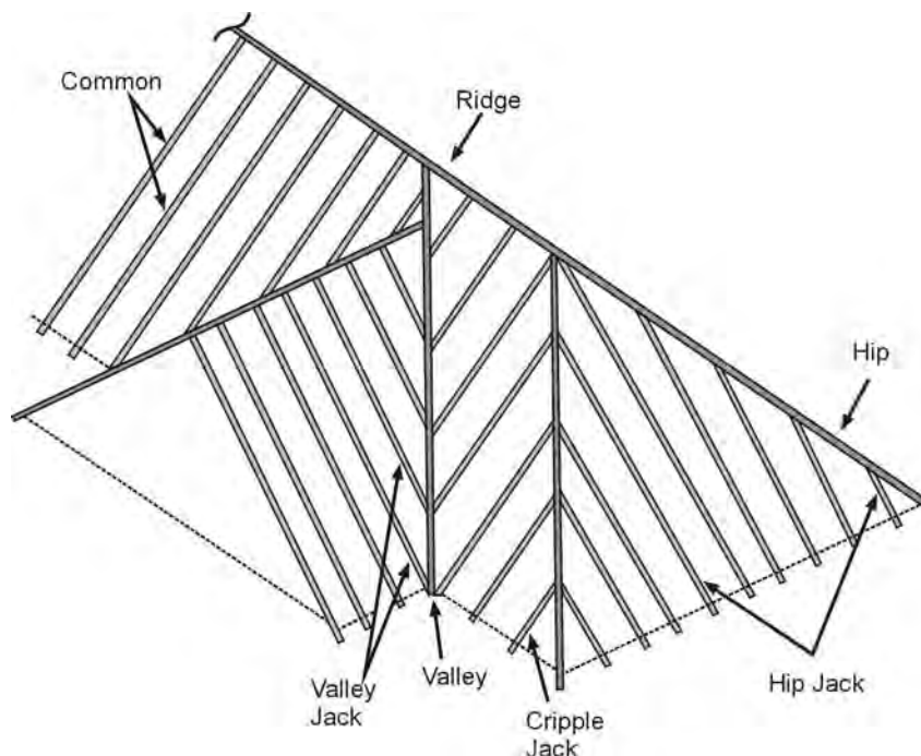
Figure 9 Roof structures
